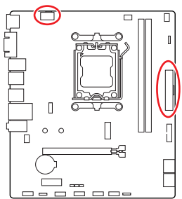
CPU_PWR1
