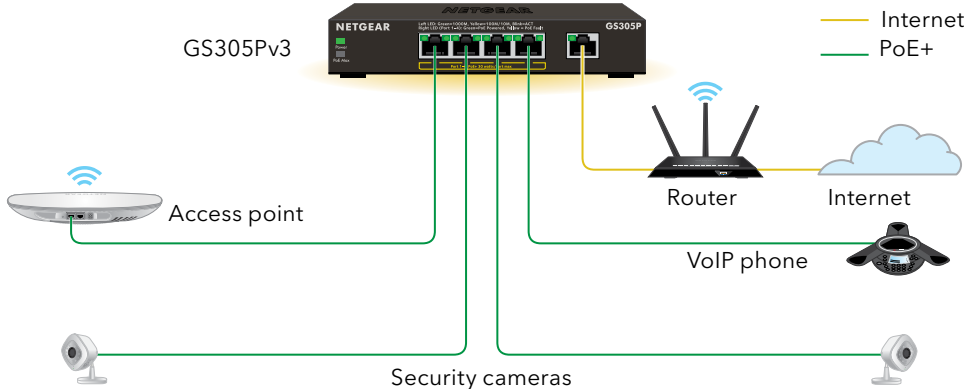
Sample connections
