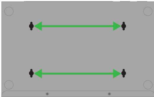
Figure 7. VESA holes at the bottom panel
