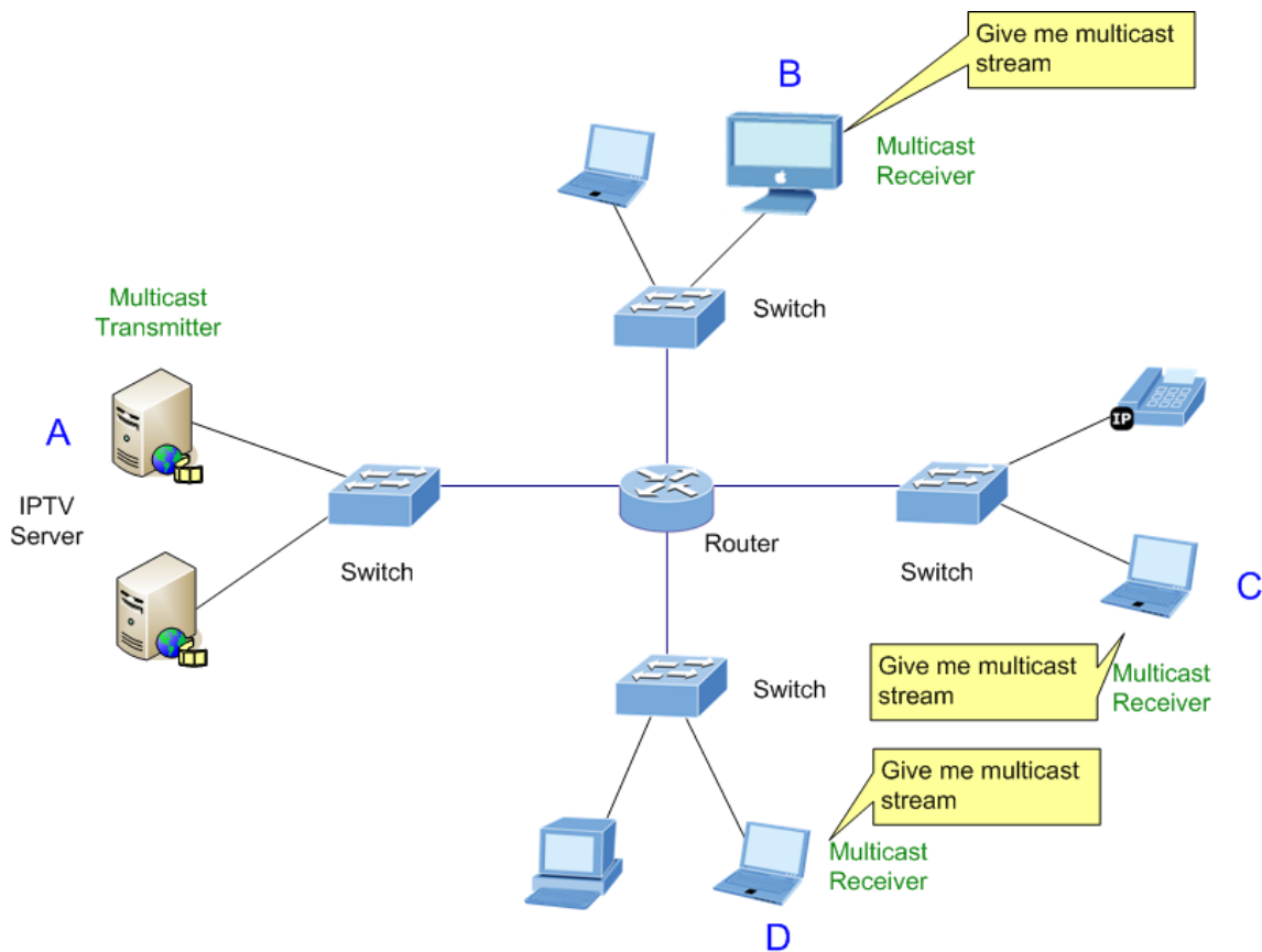
Figure 4-12-1 Multicast Service
