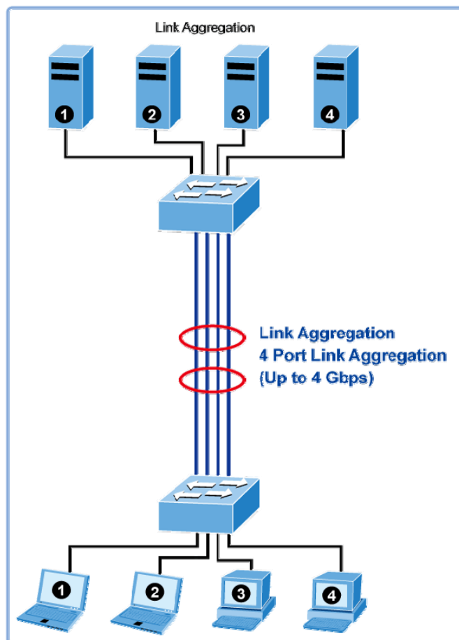
Figure 4-8-1 Link Aggregation
