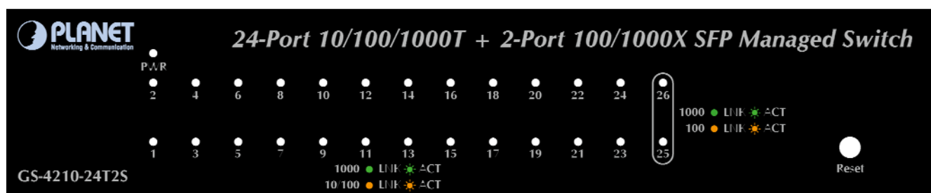
Figure 2-1-5: GS-4210-24T2S LED Panel
