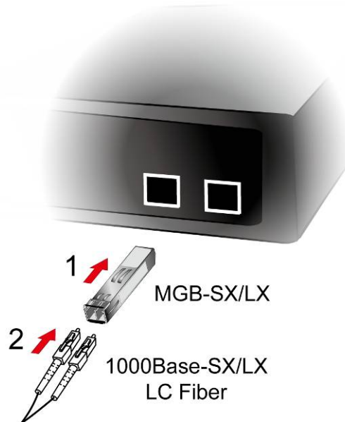
Figure 2-1-2e Plug in the SFP transceiver
