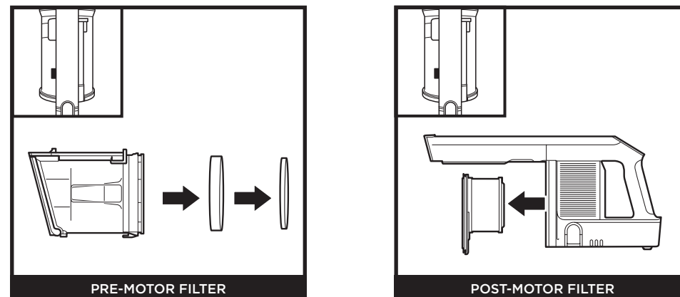
PRE-MOTOR FILTER
