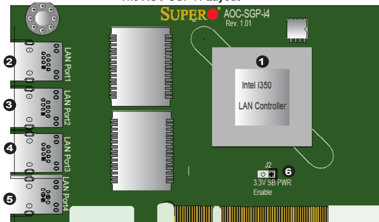
The AOC-SGP-i4 Layout
