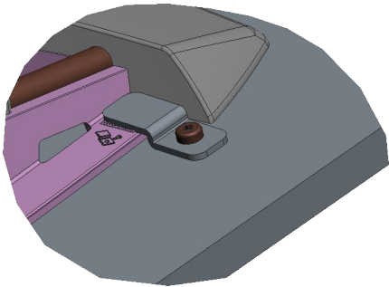
DETAIL A SCALE 0.500
