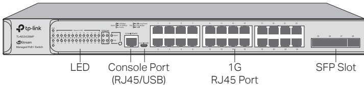
Figure 1-5 Front Panel of TL-SG3428MP
