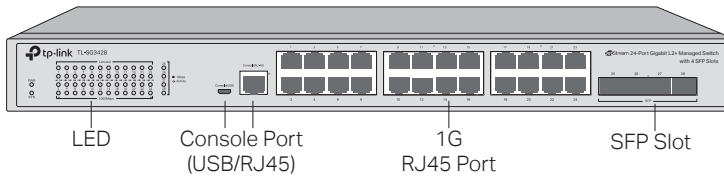
Figure 1-4 Front Panel of TL-SG3428
