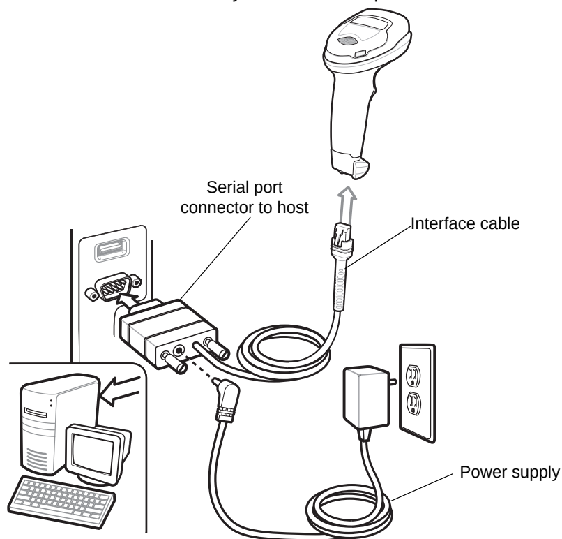
Figure 8-1 RS-232 Connection
