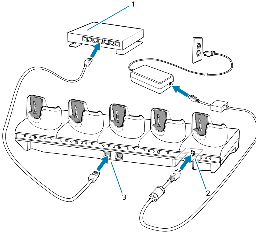
Figure 34 5-Slot Ethernet Cradle
