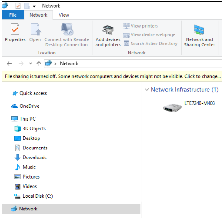
Figure 81 Network Connections
