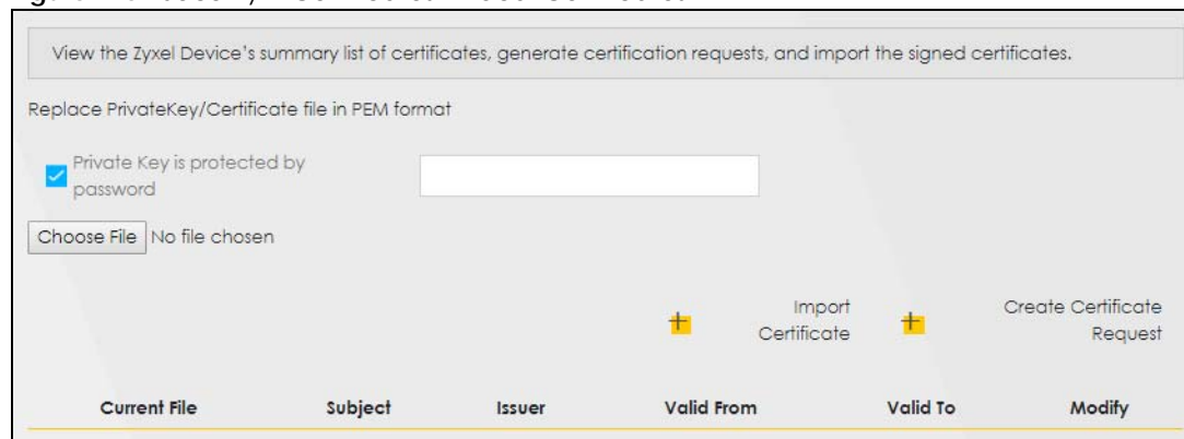
Figure 115 Security > Certificates > Local Certificates
