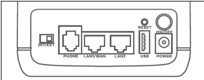
Figure 13 Rear Panel (LTE5388-M804 / LTE5398-M904)
