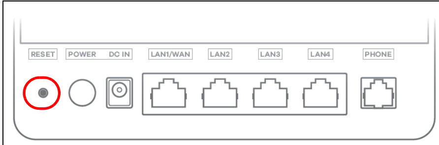
Figure 26 Reset Button (LTE3316-M604)
