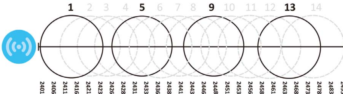
Figure 62 An Alternative Four-Channel Deployment
