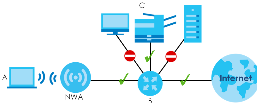
Figure 97 Layer-2 Isolation Application
