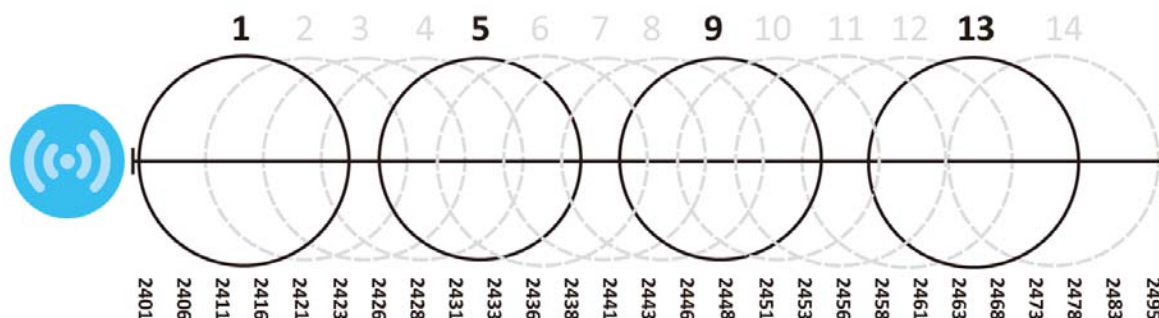
Figure 75 An Alternative Four-Channel Deployment
