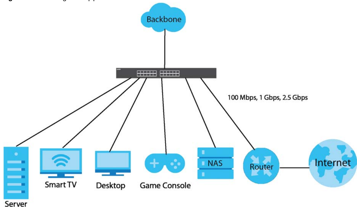
Figure 1 Multi-Gigabit Application
