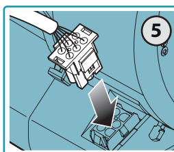
Connettore comandi Panel control connector
