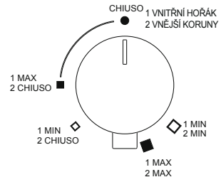
Obr. 13: knoflík hořáku dual (GIOTTO/VULCANO)
