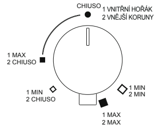
Obr. 13: knoflík hořáku dual (GIOTTO/ULCANO)
