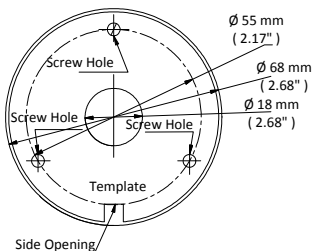
Figure 2-1 Drill Template
