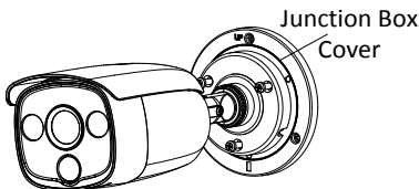
Figure 2-12 Install the Junction Box
