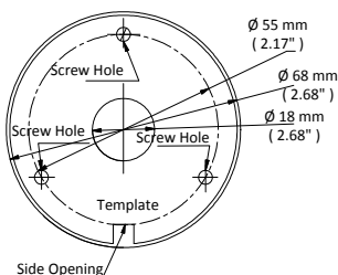
Figure 2-8 Drill Template
