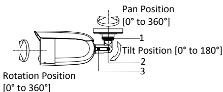
Figure 2-10 3-Axis Adjustment
