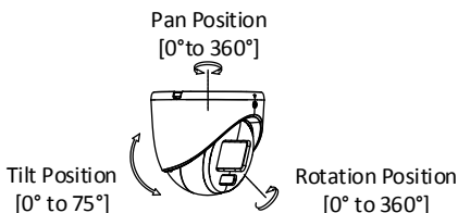
Figure 2-27 3-Axis Adjustment
