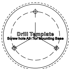
Figure 2-24 Drill Template
