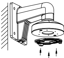
Figure 2-21 Fix the Gang Box
