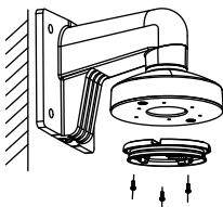
Figure 2-36 Fix the Wall Mount
