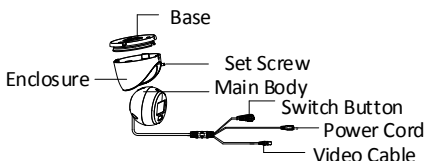
Figure 1-4 Overview of Type IV Camera
