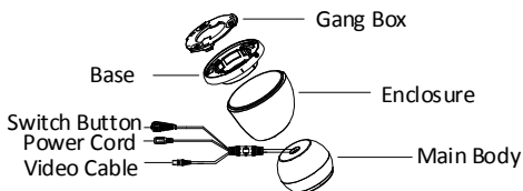
Figure 1-3 Overview of Type III Camera
