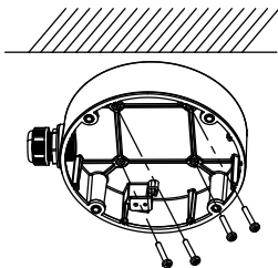
Figure 2-47 Secure the Junction Box Body
