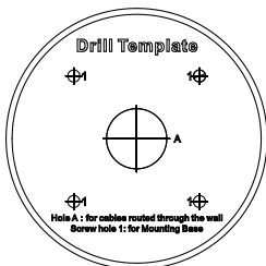
Figure 2-43 Drill Template
