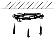
Figure 2-12 Attach the Gang Box to the Ceiling
