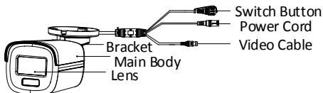
Figure 1-2 Overview of Type II Camera
