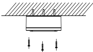
Figure 2-31 Combine the Junction Box Cover and Body
