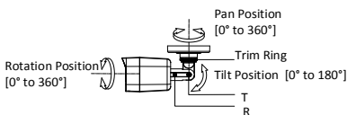
Figure 2-2 3-Axis Adjustment
