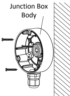
Figure 2-4 Secure the Junction Box on the Wall/Ceiling
