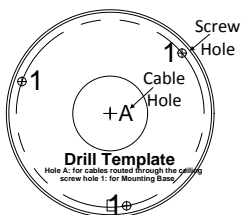
Figure 2-14 Drill Template
