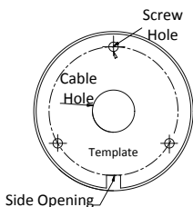
Figure 2-1 Drill Template
