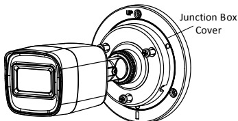
Figure 2-5 Fix the Camera on the Junction Box's Cover
