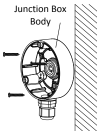
Figure 2-6 Fix the Junction Box to the Wall/Ceiling
