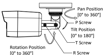
Figure 2-3 3-axis Adjustment
