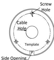
Figure 2-1 Drill Template
