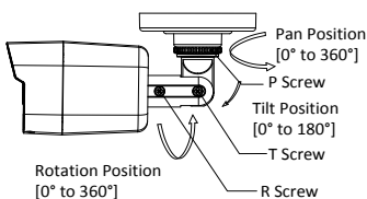
Figure 2-3 3-axis Adjustment
