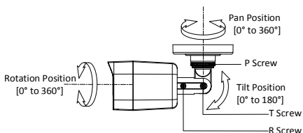
Figure 2-3 3-axis Adjustment
