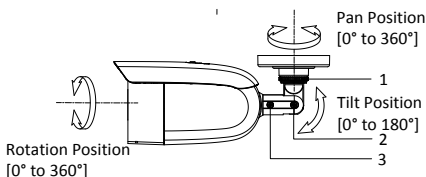
Figure 2-10 3-Axis Adjustment
