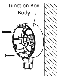
Figure 2-6 Fix the Junction Box to the Wall/Ceiling
