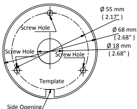
Figure 2-1 Drill Template
