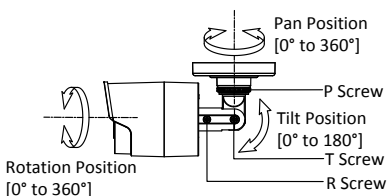
Figure 2-3 3-axis Adjustment
