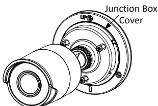
Figure 2-5 Fix the Camera on the Junction Box's Cover
