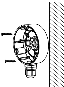
Figure 2-12 Install the Junction Box
