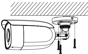
Figure 2-9 Fix the Camera to the Ceiling
