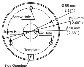
Figure 2-8 Drill Template
