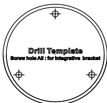
Figure 2-11 Drill Template
