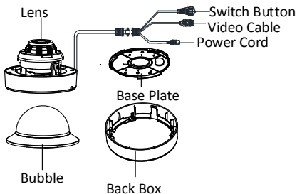
Figure 1-2 Overview of Type II Camera
