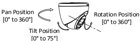
Figure 2-42 3-Axis Adjustment
