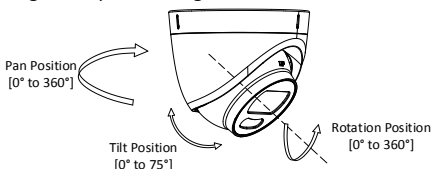
Figure 2-16 3-Axis Adjustment
