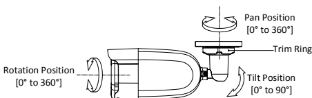
Figure 2-10 3-Axis Adjustment
