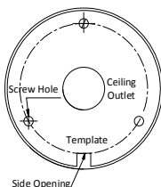
Figure 2-8 Drill Template
