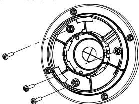
Figure 2-18 Secure screws on the Junction Box's Cover
