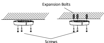
Figure 2-14 Attach the Mounting Base to the Ceiling
