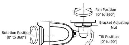
Figure 2-3 3-Axis Adjustment
