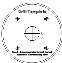
Figure 2-17 Drill Template
