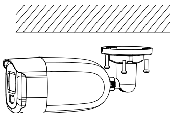
Figure 2-9 Secure the Camera to the Ceiling
