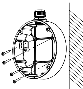
Figure 2-19 Secure the Junction Box's Body
