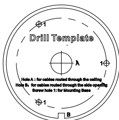
Figure 2-13 Drill Template
