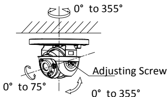
Figure 2-14 Type III Camera 3-Axis Adjustment
