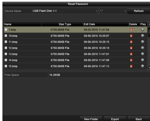
Figure 17-19 Export GUID
