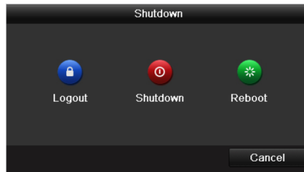
Figure 2-35 Logout
