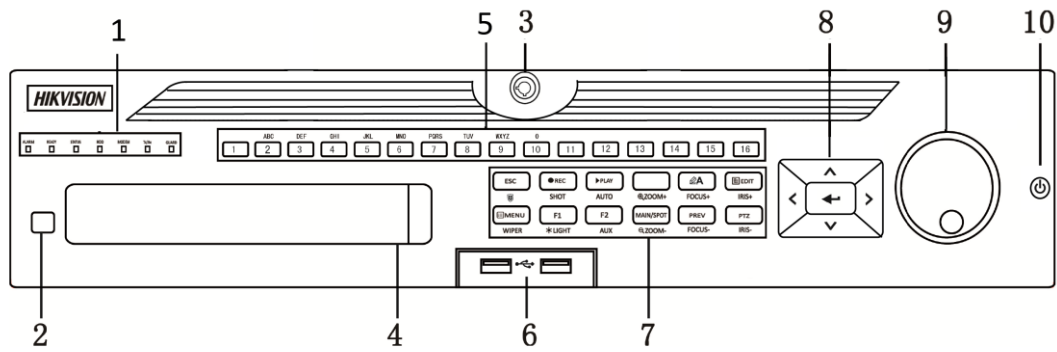
Figure 1-7 Front Panel of DS-9000HUHI-F8/N
