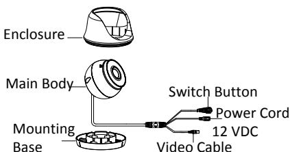
Figure 1-5 Overview of Type V Camera
