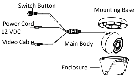
Figure 1-3 Overview of Type III Camera
