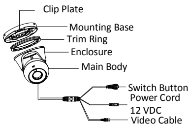
Figure 1-4 Overview of Type IV Camera
