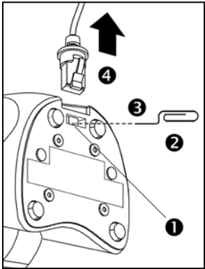
Figure 2. Cable Release
