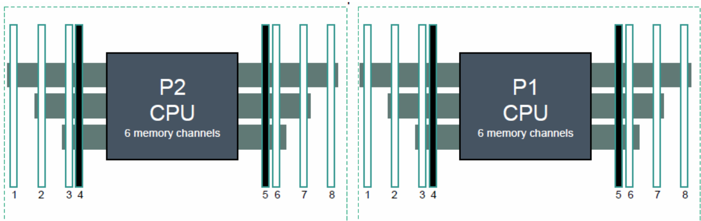
HPE DL160/Gen10 Servers Front Server (2+1+1 slots per channel)
