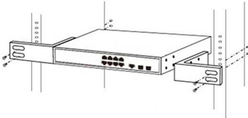
Figure 6 - Rack Installation
