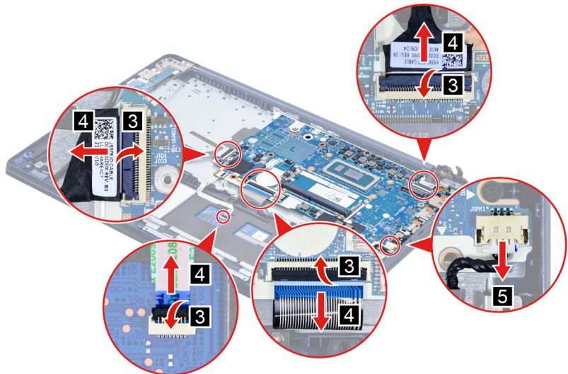
Figure 48. Disconnect cables
