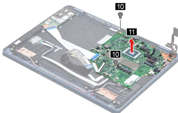
Figure 29. Remove the system board
