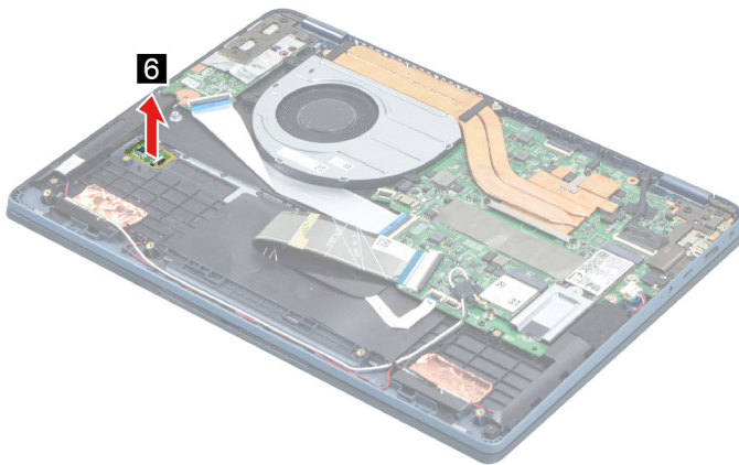
Figure 21. Remove fingerprint board
