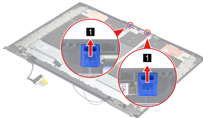
Figure 32. Remove the microphone rubbers
