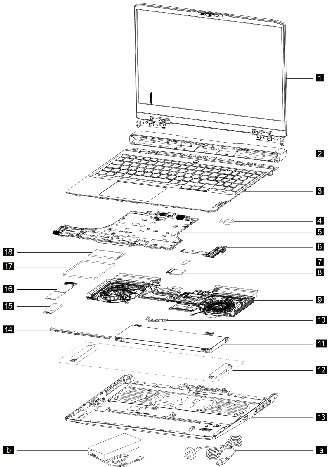
Figure 1. IdeaPad Gaming 3 series exploded view
