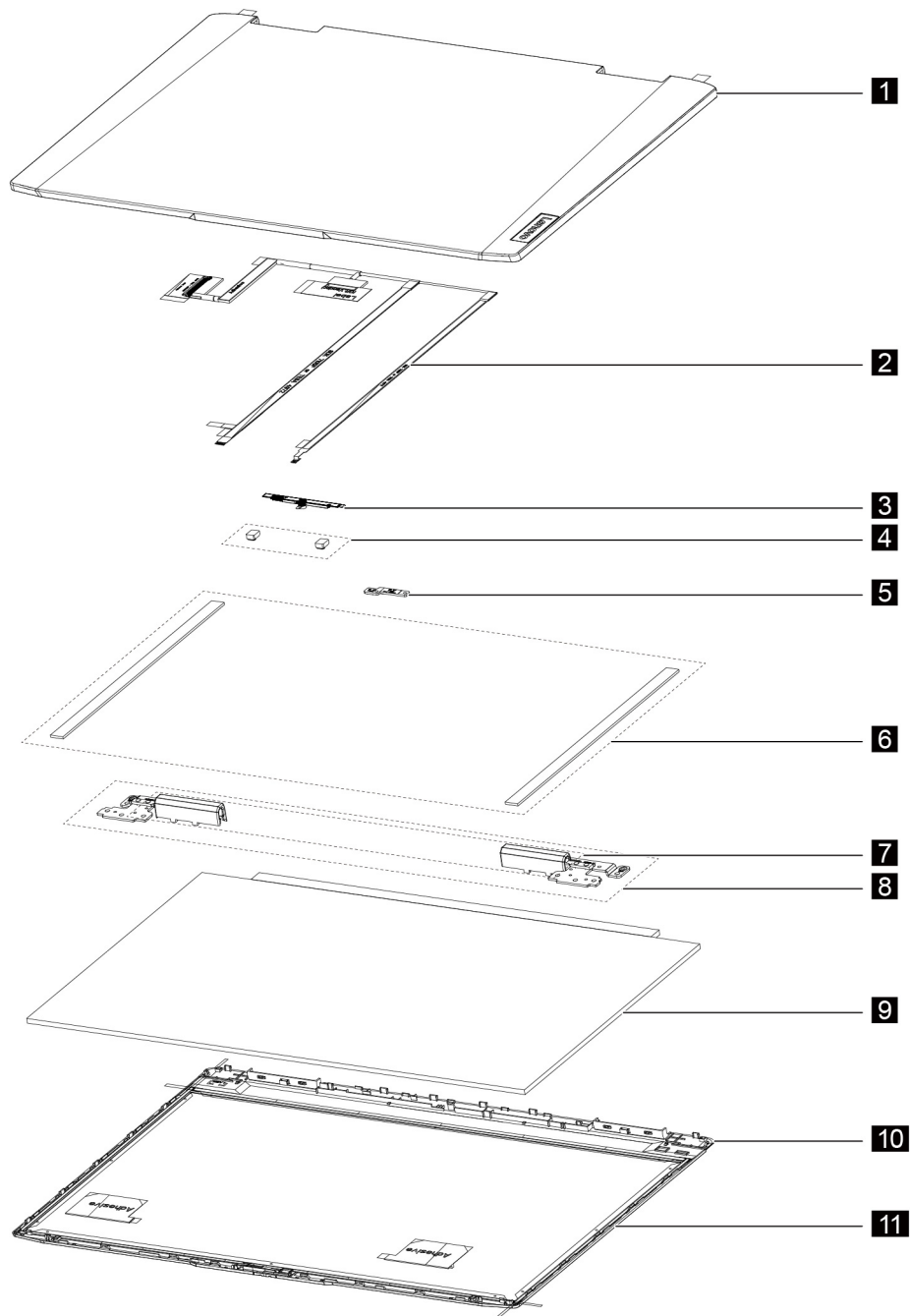
Figure 2. IdeaPad Gaming 3 series LCD module — exploded view
