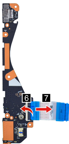
Figure 25. Remove the I/O board cable
