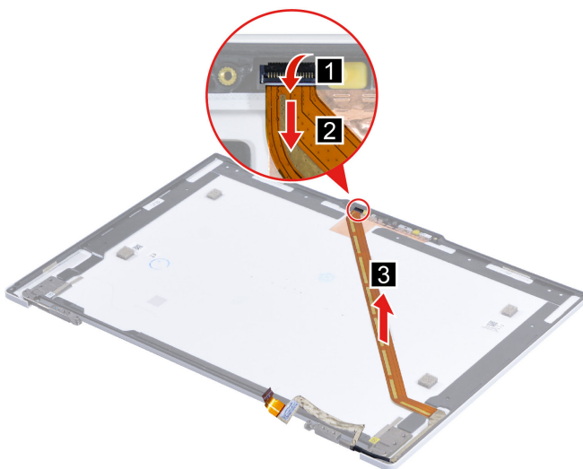
Figure 40. Remove the camera cable
