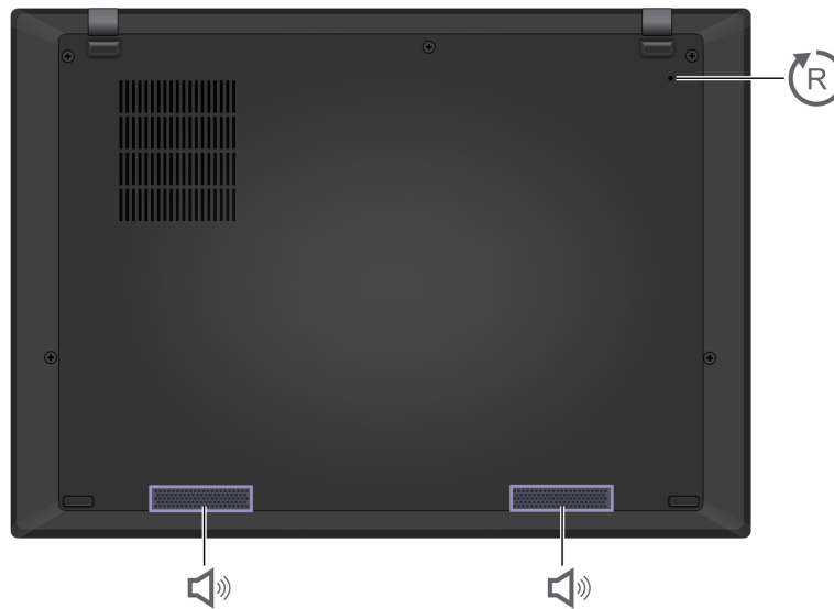
Emergency-reset hole
