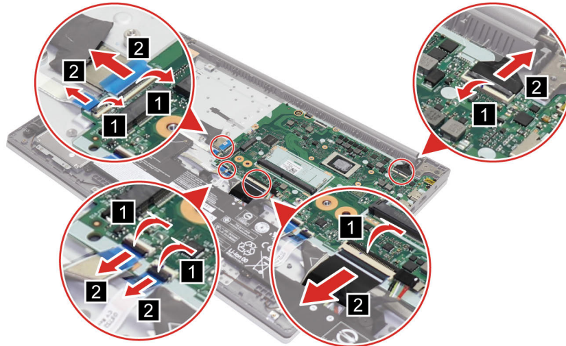
Figure 31. Disconnect cables
