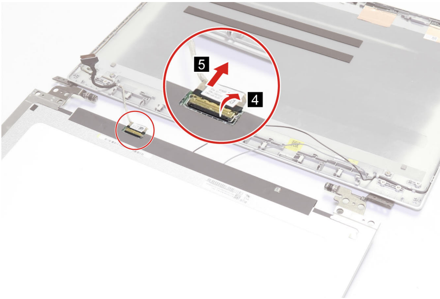
Figure 42. Disconnect the EDP cable
