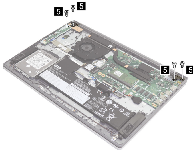
Figure 35. Remove four screws
