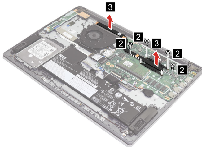
Figure 13. Loosen four screws and remove the heat sink
