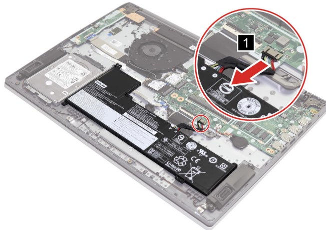
Figure 8. Disconnect the battery pack cable
