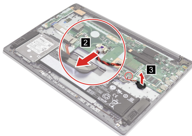
Figure 20. Disconnect the coin-cell battery cable and remove the coin-cell battery
