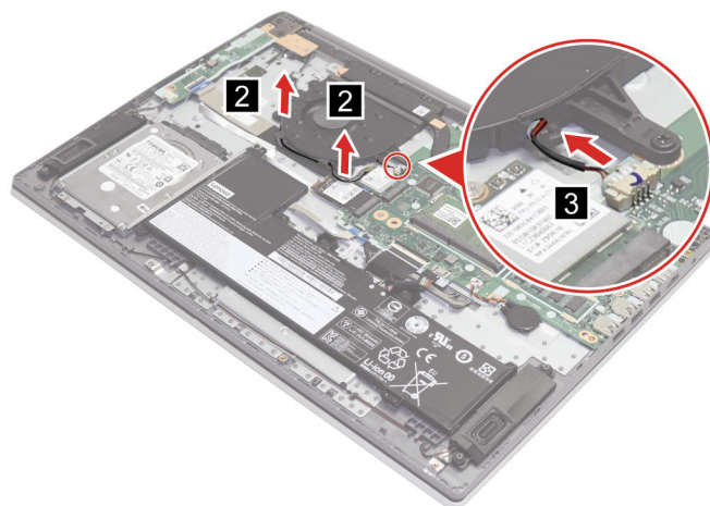
Figure 15. Disconnect the fan cables
