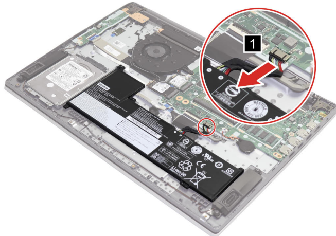
Figure 6. Disconnect the battery pack cable
