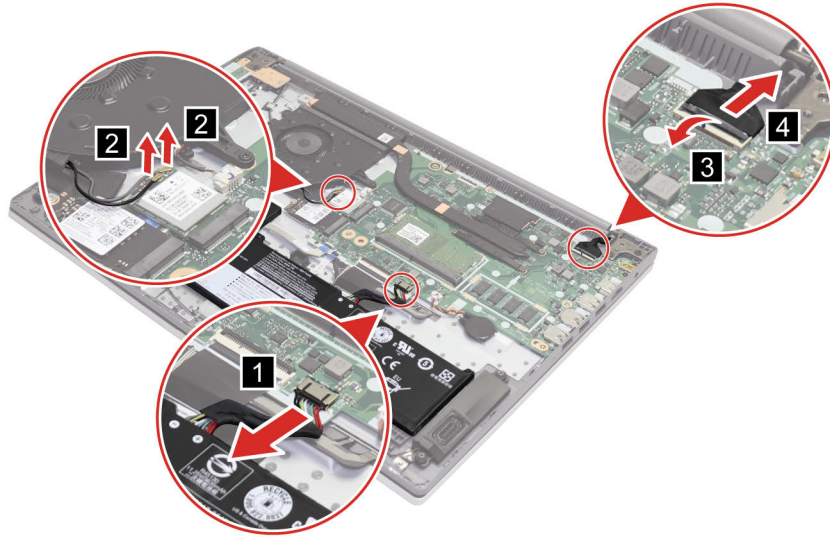
Figure 34. Disconnect battery pack cables, EDP cable, and antenna cables
