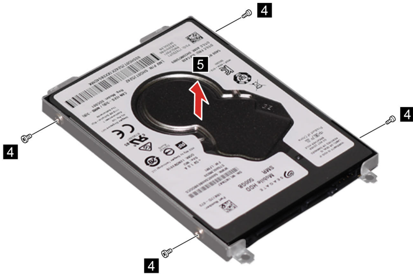
Figure 11. Remove four screws and remove the storage drive
