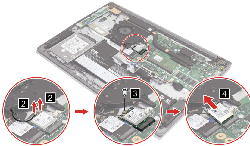
Figure 24. Remove one screw and slide the Wi-Fi card out of the slot
