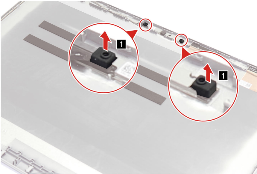
Figure 46. Remove the microphone rubber
