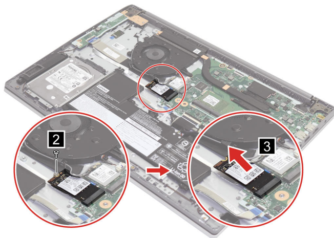
Figure 18. Remove one screw and slide the solid-state drive out of the slot
