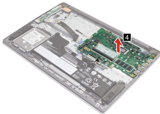
Figure 33. Remove the system board
