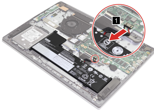
Figure 23. Disconnect the battery pack cable
