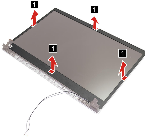
Figure 39. Remove the LCD bezel
