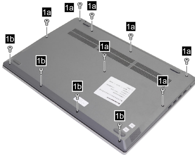
Figure 4. Remove eleven screws
