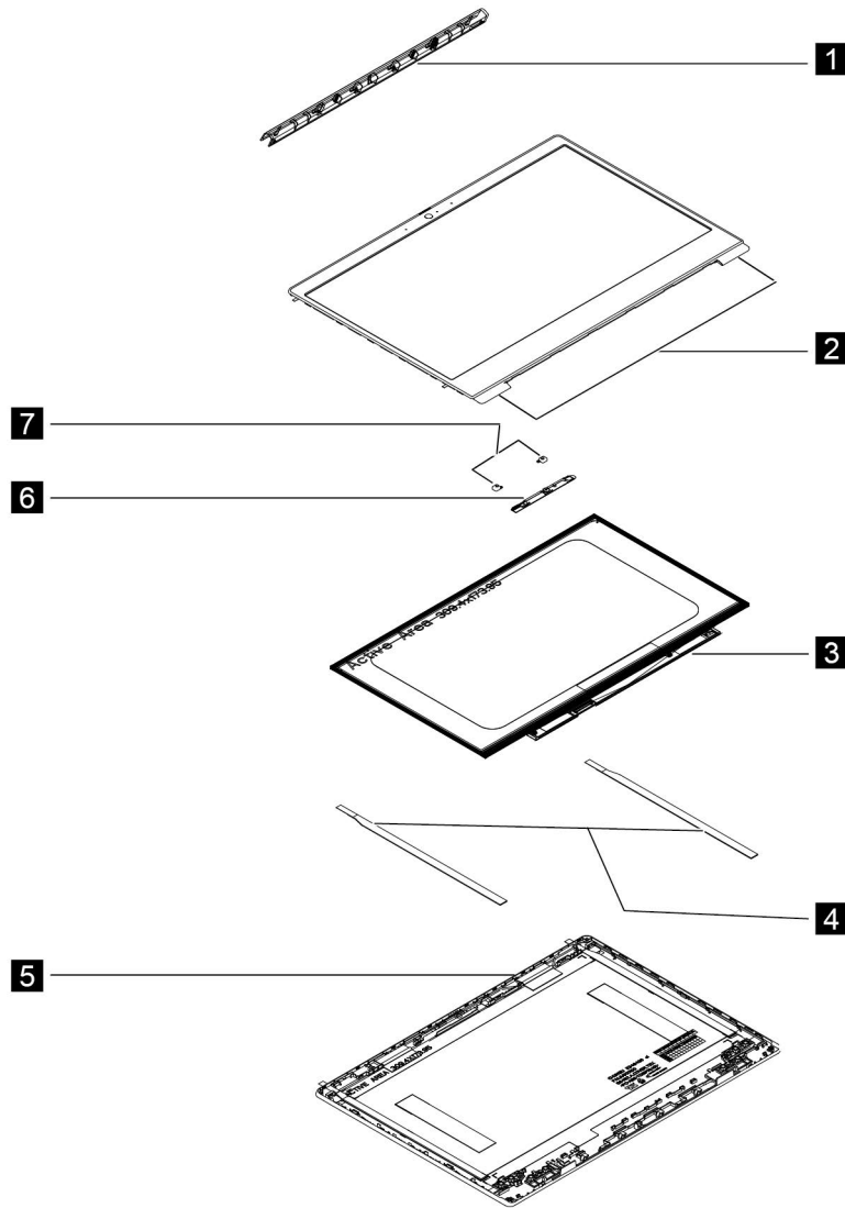
Figure 2. Lenovo V17-IIL LCD exploded view
