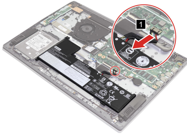
Figure 17. Remove the battery pack cable
