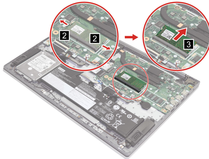
Figure 22. Disengage the latch and slide the memory module out of the slot
