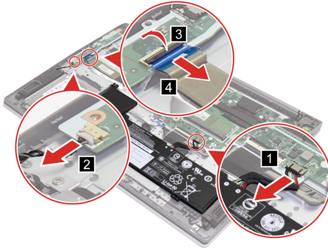
Figure 27. Disconnect cables from the I/O board
