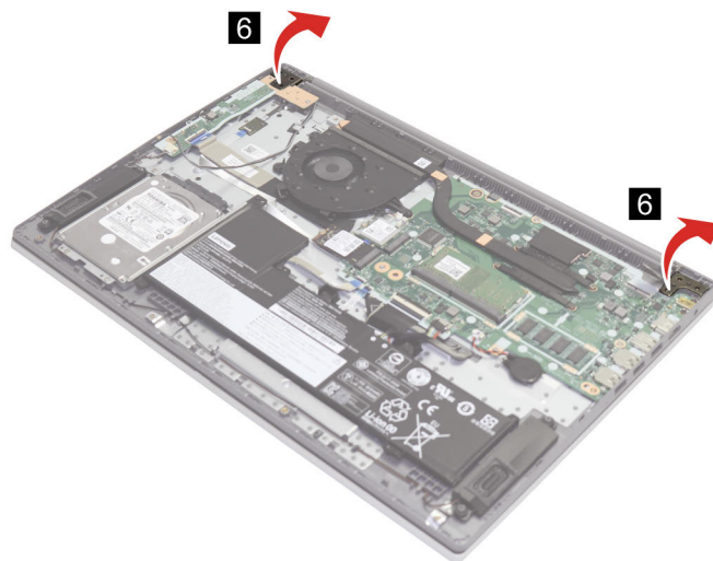
Figure 36. Open the hinges
