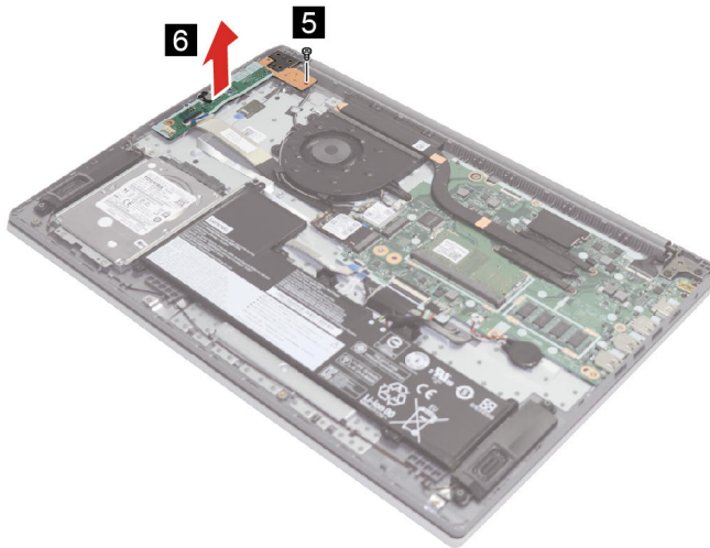
Figure 28. Remove the screw and then remove the I/O board
