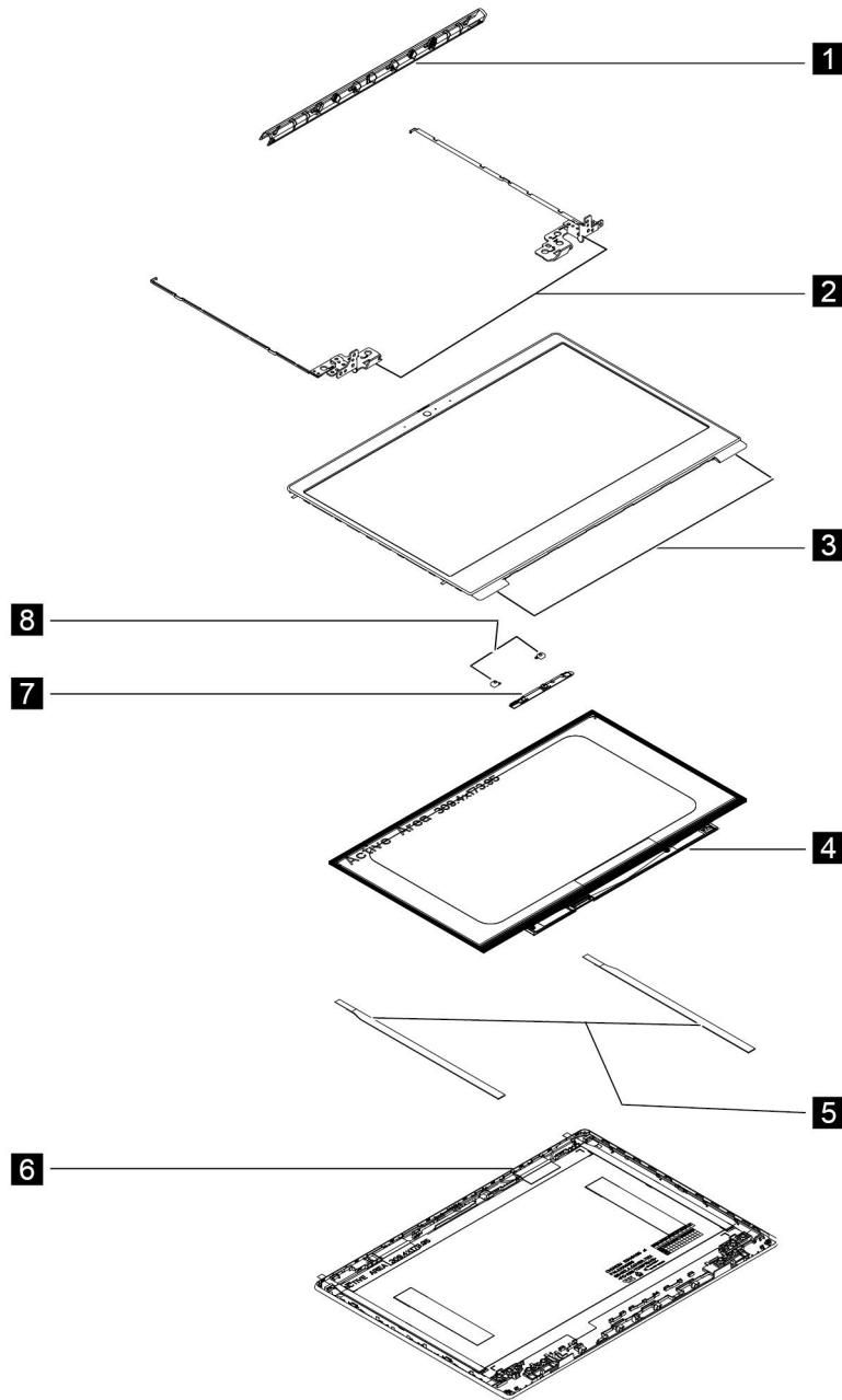
Figure 1. Lenovo V14 Gen1 i and Lenovo V15 Gen1 i LCD exploded view
