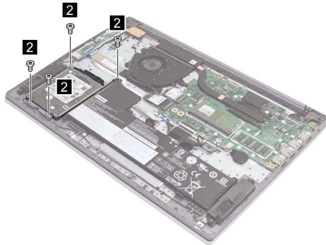
Figure 9. Remove four screws
