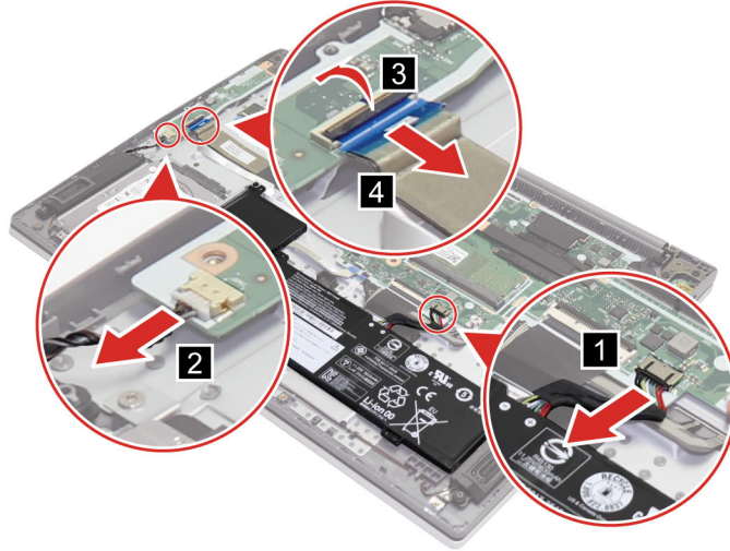
Figure 25. Disconnect cables from the I/O board
