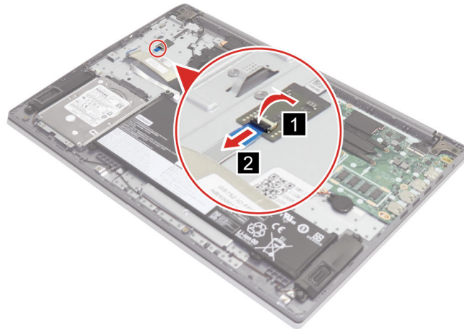
Figure 29. Disconnect the fingerprint board cable
