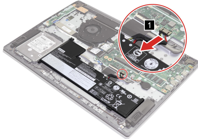
Figure 19. Disconnect the battery pack cable
