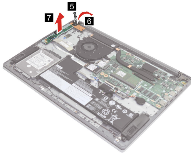
Figure 26. Remove the screw and then remove the I/O board
