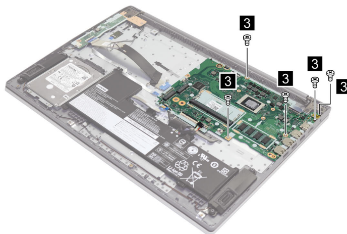
Figure 32. Remove five screws
