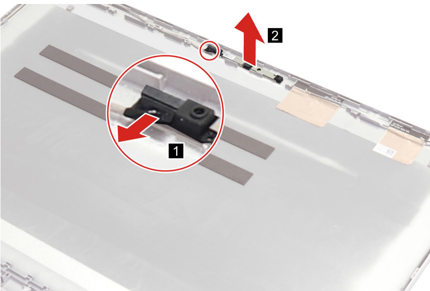
Figure 47. Disconnect the camera module cable and remove the camera module
