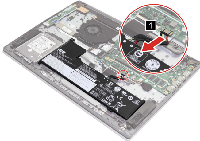
Figure 14. Remove the battery pack cable
