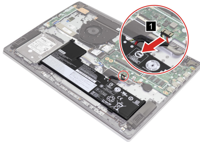
Figure 12. Disconnect the battery pack cable
