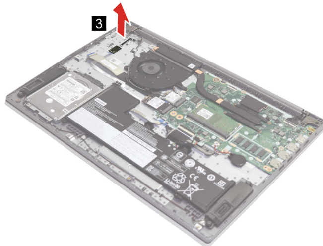
Figure 30. Remove the fingerprint reader
