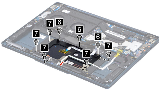
Figure 25. Remove eight screws
