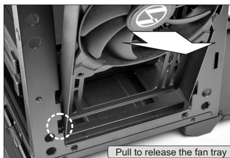
Pull to release the fan tray
