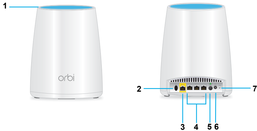
Figure 4. Orbi router model RBR40, front and back views
