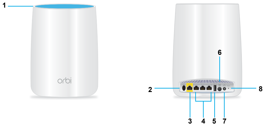
Figure 2. Orbi router model RBR50, front and back views
